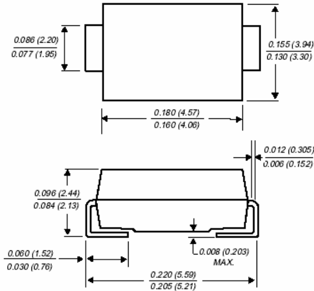
Dimensions in inches and (millimeters) DO-214AA(SMB)
